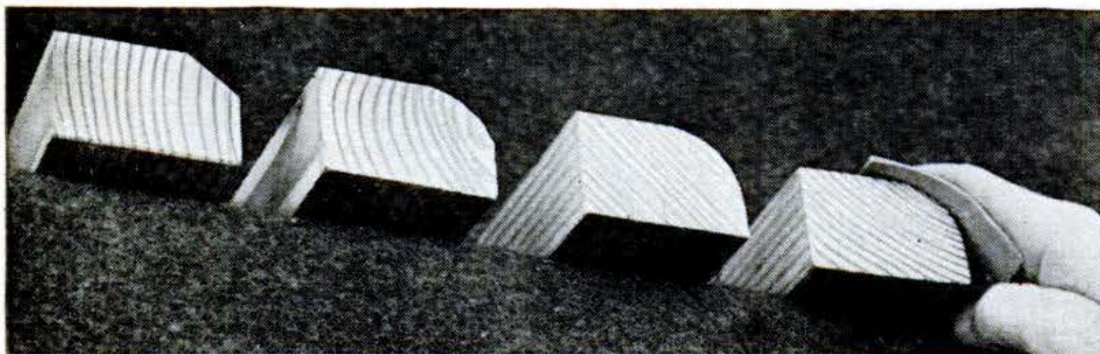
ROUNDING BY HAND: Plane corner to 45°, reduce high spots of angle by more planing, and finish by hand. Built-up corner is at right.
